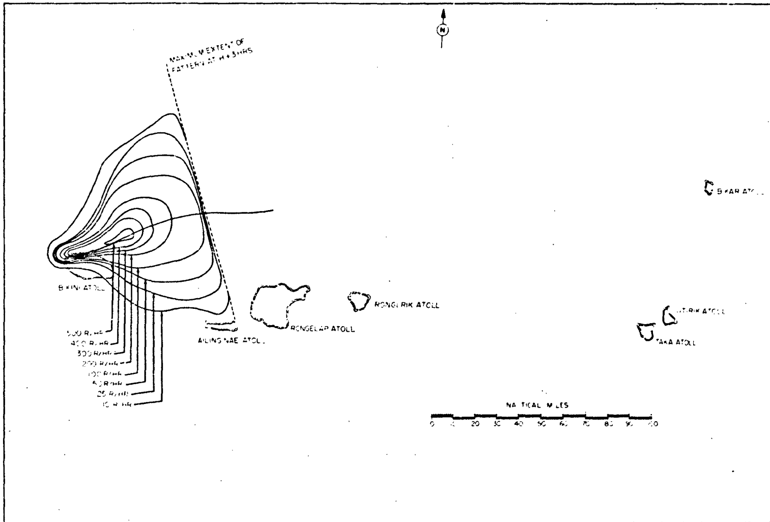
Fig. 6.9 Shot 1, reconstructed Fallout Pattern at 3 hr
