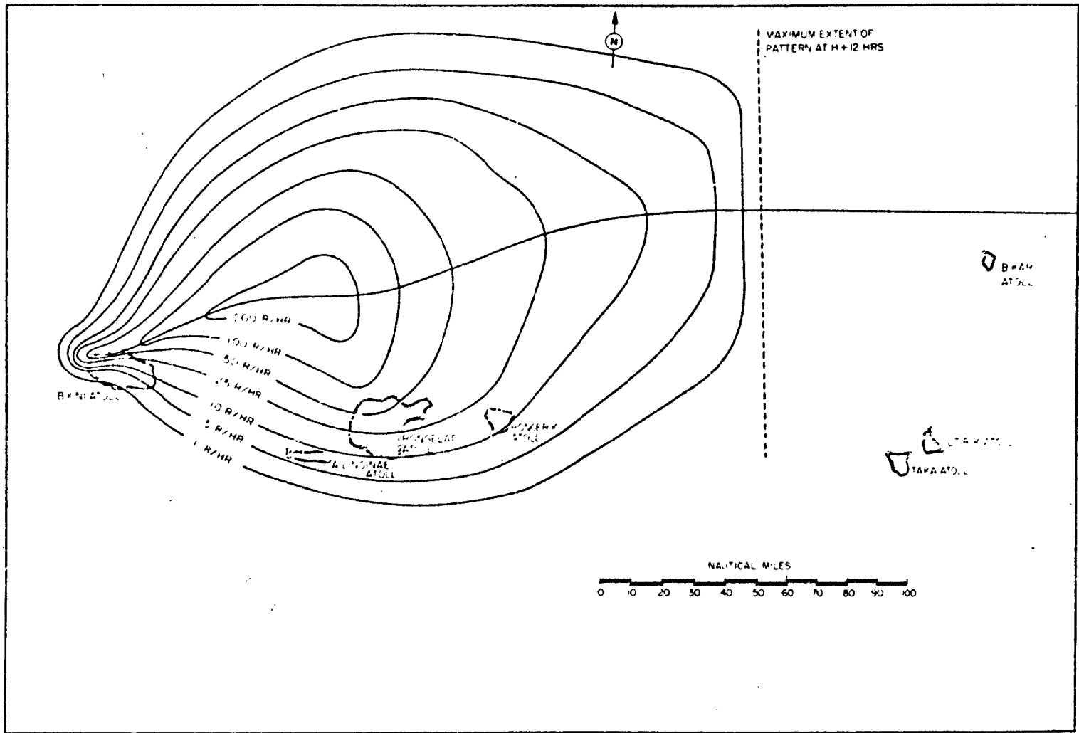
Fig. 6.11 Shot 1, Reconstructed Fallout Pattern at 12 hr
