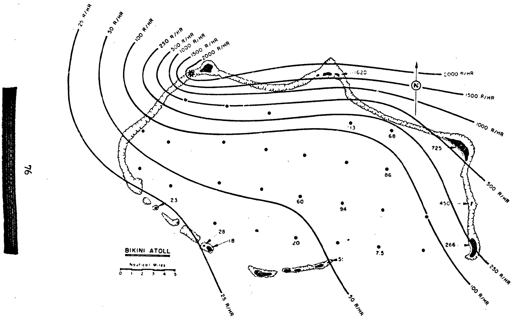
Fig. 6.1 Shot 1, Close-in Gamma Fallout Pattern (r/hr at 1 hr)
