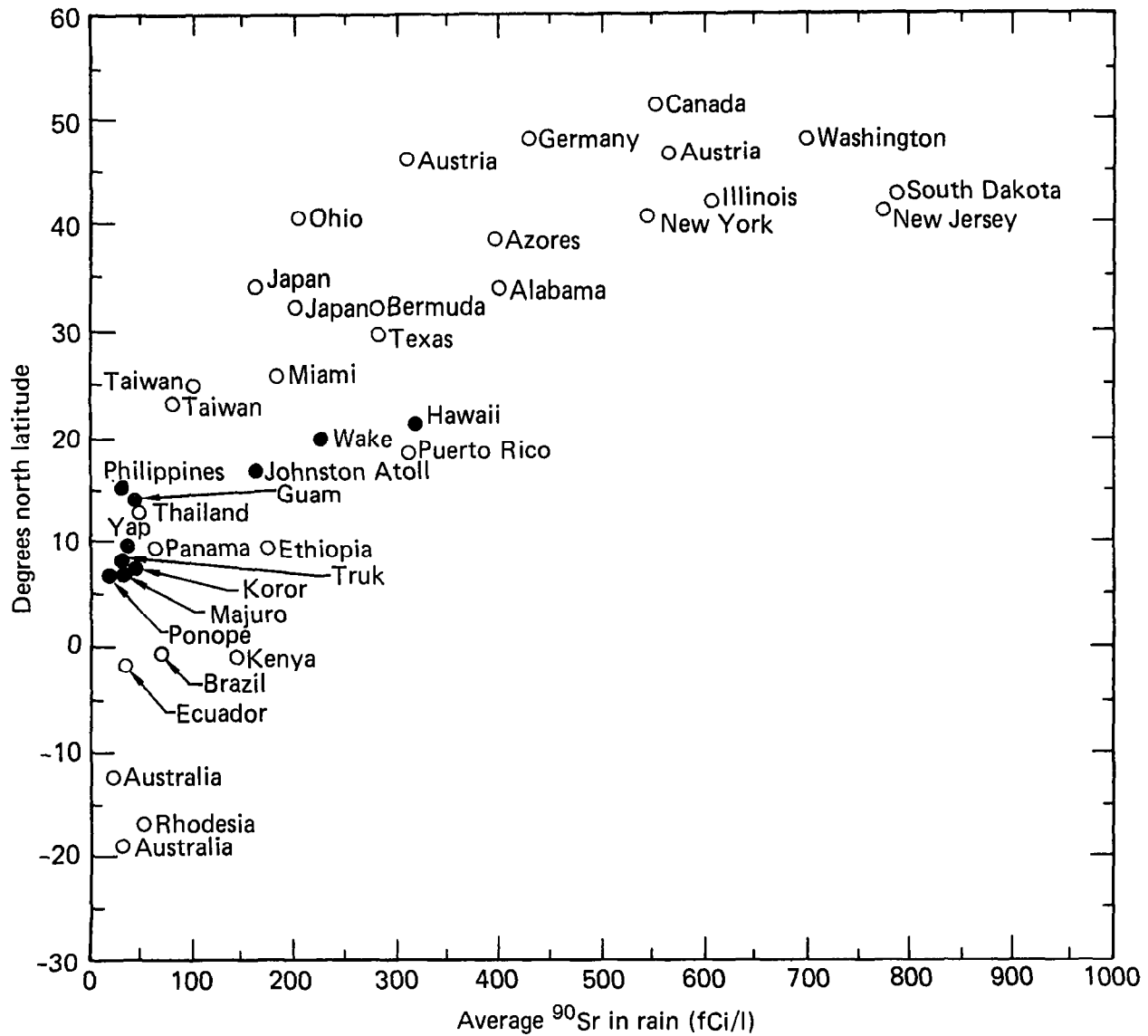
FIG. 2. The average ^{90}\text{Sr} in rain from 1976 to the fourth quarter of 1978 as a function of latitude.
