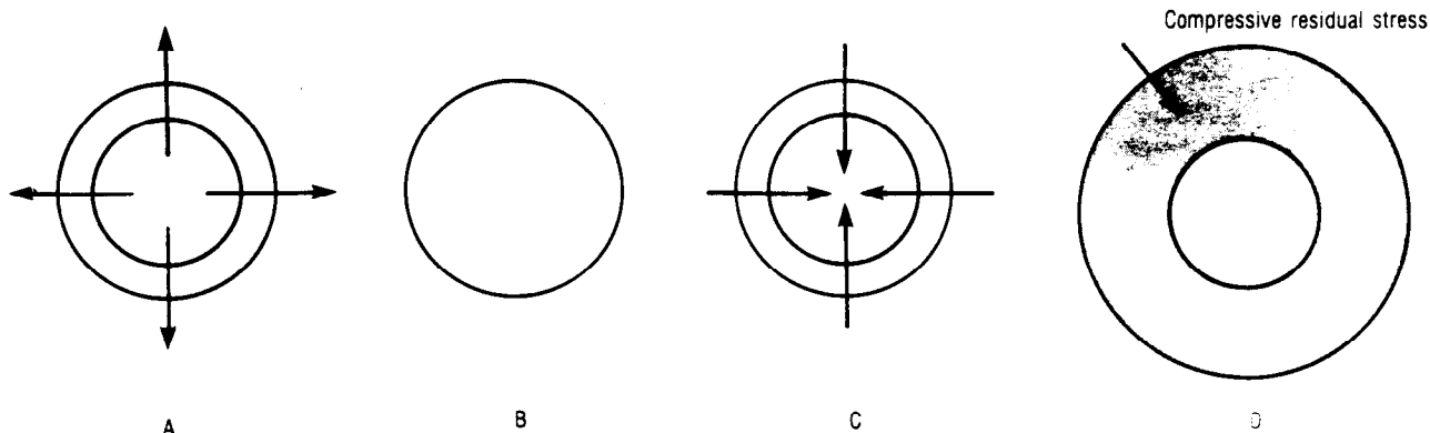
Figure 3-1—Formation of Stress "Containment Cage"
