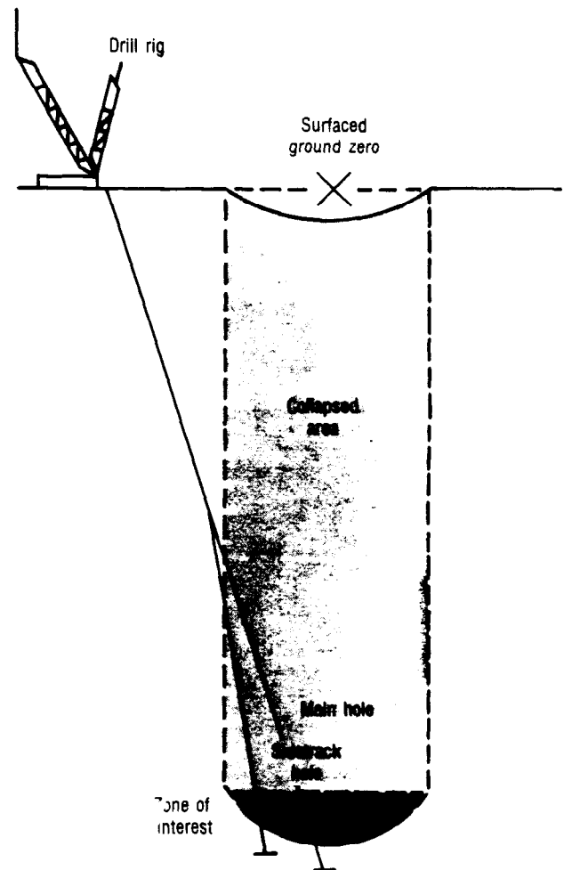
Figure 2-3—Drill-Back Operation
