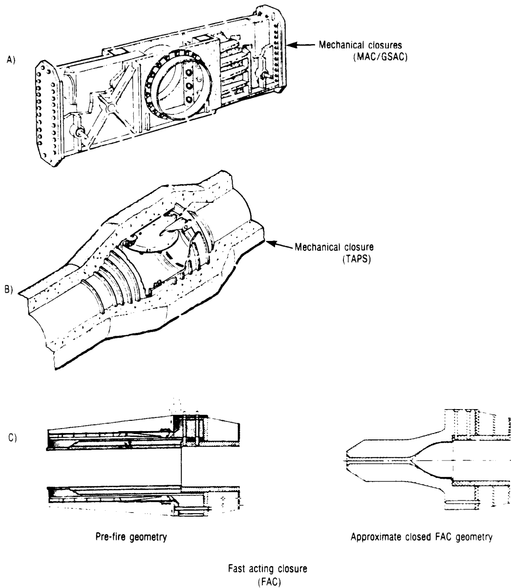
Figure 3-7—Vessel Closures
