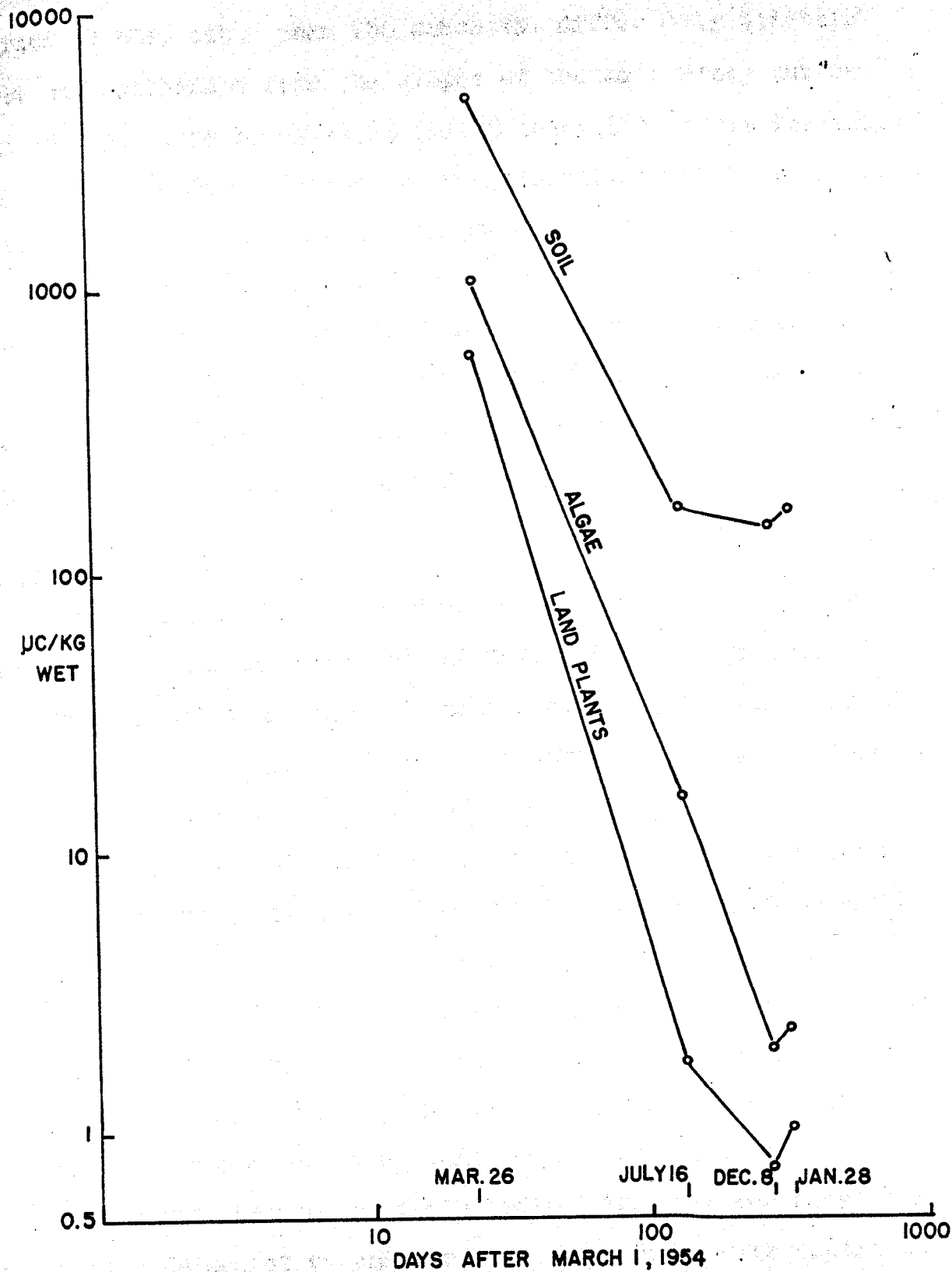
FIG. 9 RATE OF DECLINE IN LAND PLANTS , ALGAE AND SOIL SAMPLES AT KABELLE 1954 — 1955
