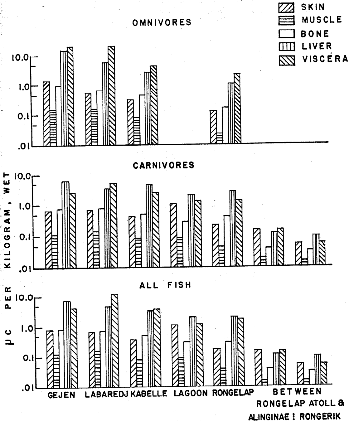
FIG. 5 RADIOACTIVITY IN MICROCURIES PER KILOGRAM IN FISH TISSUES COLLECTED IN THE VICINTY OF RONGELAP ATOLL, DECEMBER 1954 AND JANUARY 1955
