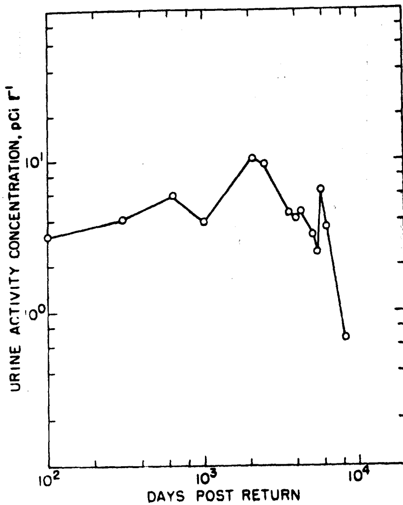
Fig. 4 Mean Adult 90 Sr Urine Activity Concentration History at Rongelap Atoll
