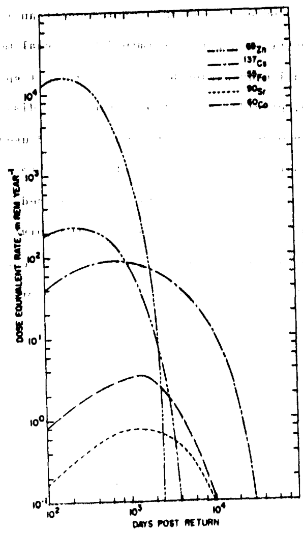
Fig. 17 Adult Mean Total Body Dose Equivalent Rate at Utirik Atoll Post Mid 1954
