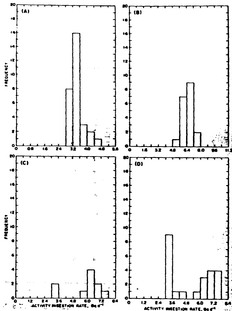
Fig. 13b 90 Sr Daily Activity Ingestion Rate for (A) Adult Males (B) Adult Females (C) Young Adults and (D) Children on Rongelap
