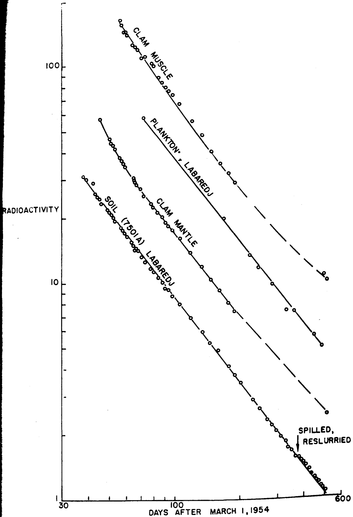
FIG. 12 LOG-LOG PLOTS OF RONGELAP DECAY SAMPLES OF MARCH 26, 1954: PLANKTON FROM LABAREDJ; MUSCLE AND MANTLE OF GIANT CLAM, HIPPUPUS , FROM KABELLE; AND SOIL ON WHICH DECAY CORRECTION FACTORS WERE BASED
