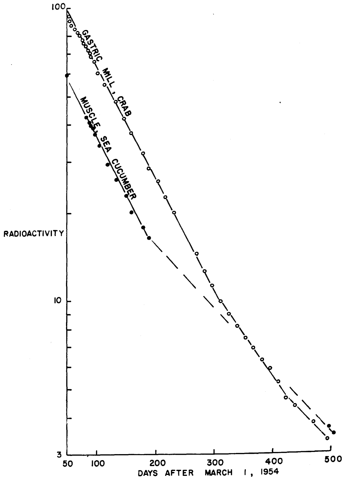
FIG. II SEMI-LOG PLOTS OF DECAY CURVES OF GASTRIC MILL OF CRAB, GRAPSUS GRAPSUS , AND MUSCLE OF SEA CUCUMBER, HOLOTHURIA ATRA COLLECTED MARCH 26, 1954 AT KABELLE
