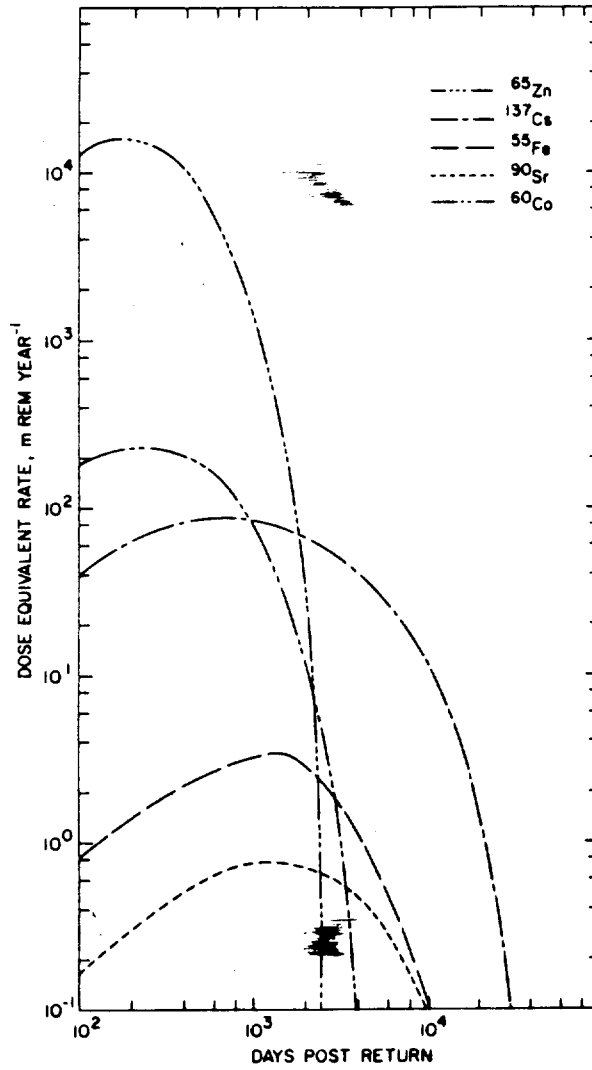
Fig. 17 Adult Mean Total Body Dose Equivalent Rate at Utiirik Atoll Post Mid-1954
