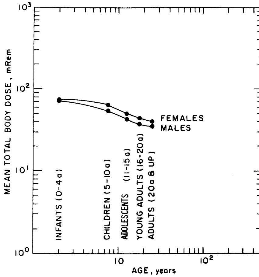
Fig. 22 Age and Sex Group Mean Values for 90 Sr Dose Equivalent for the Interval 1957 to 1980 at Rongelap Atoll
