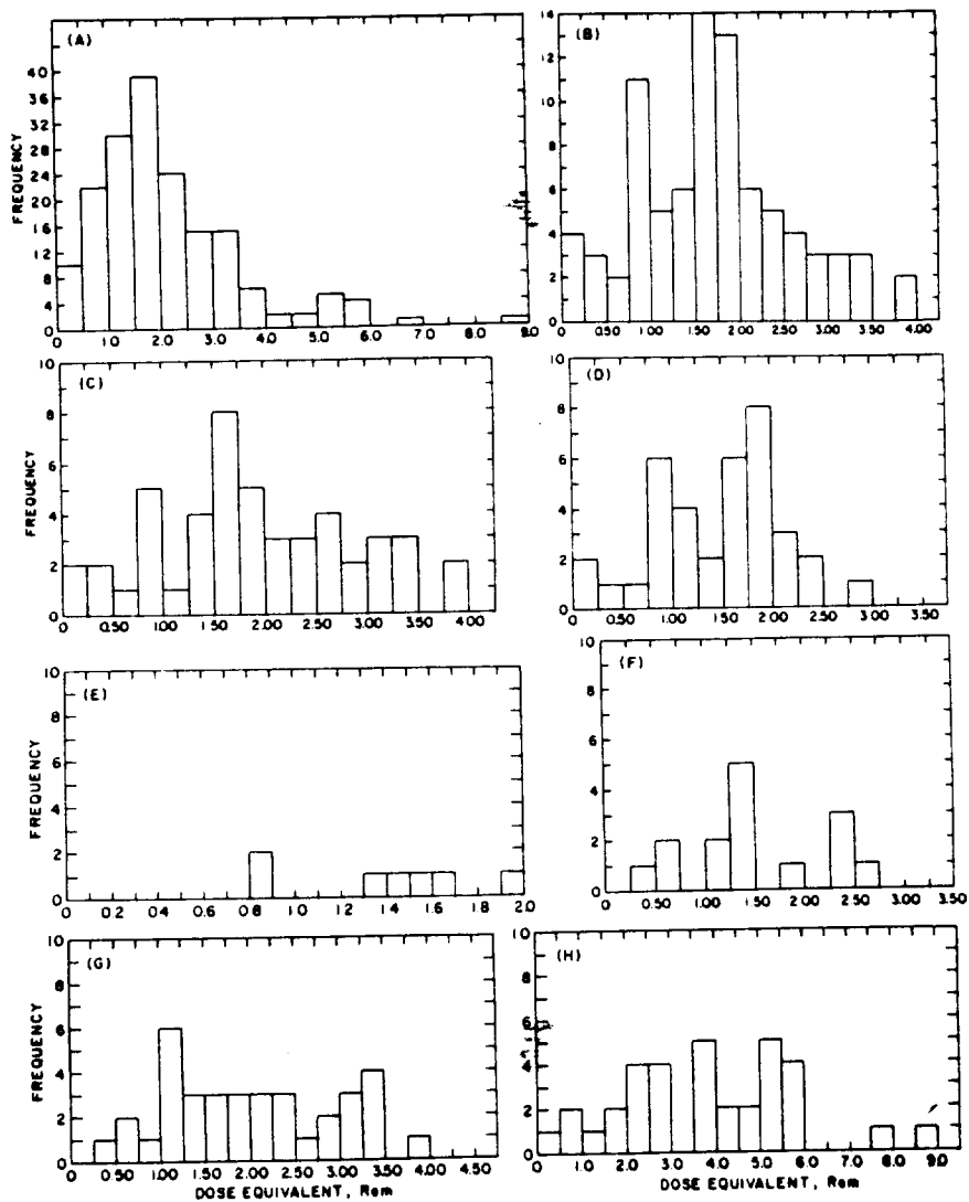
Fig. 19 ^{137}\text{Cs} Dose Equivalent to (A) All Residents (B) Adults (C) Adult Males (D) Adult Females (E) Young Adults (F) Adolescents (G) Children and (H) Infants on Rongelap.
