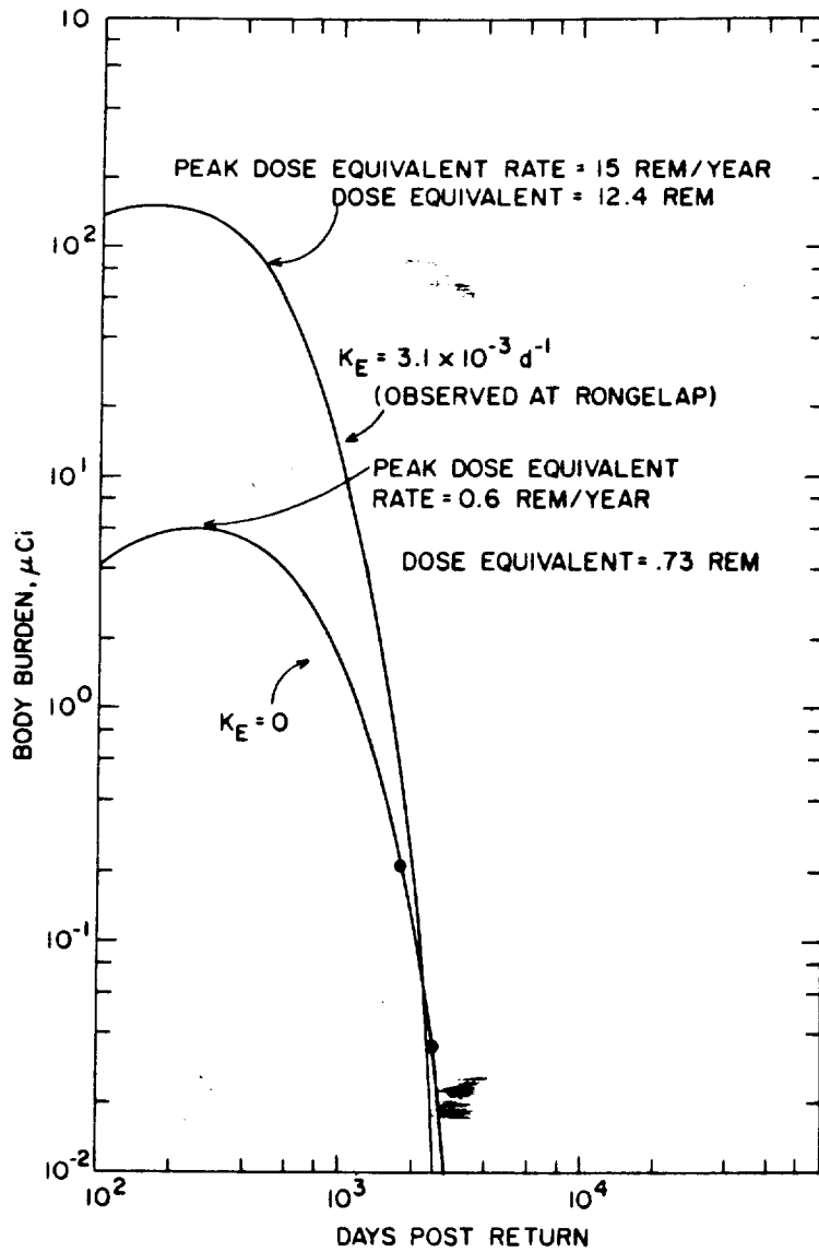
Fig. 16 Mean Adult ^{65}\text{Zn} Body Burden, Peak Dose Equivalent Rate and Dose Equivalent for Utirik Atoll
