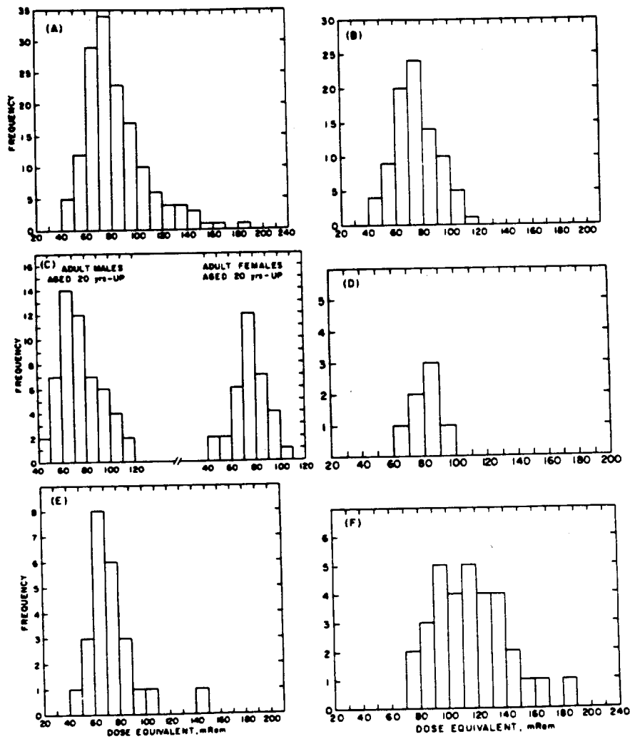
Fig 21 ^{65}\text{Zn} Dose Equivalent to (A) All Residents (B) Adults (C) Adult Males and Females (D) Adolescents (E) Children and (F) In- fants on Rongelap Atoll
