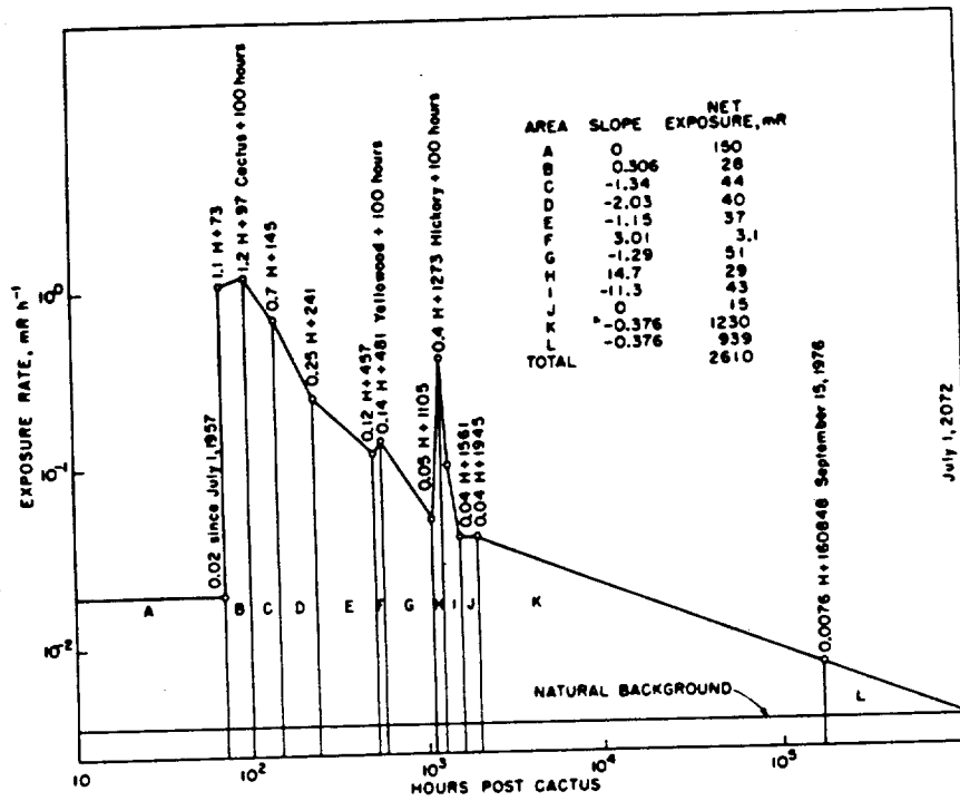
Fig 25 Rongelap External Exposure Rate History Post Cactus
