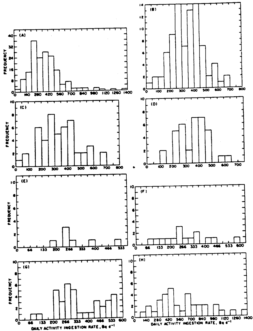
Fig. 11 137 Cs Daily Activity Ingestion Rate For (A) All Residents (B) Adults (C) Adult Males (D) Adult Females (E) Young Adults (F) Adolescents (G) Children and (H) Infants on Rongelap - Referenced to June 1957
