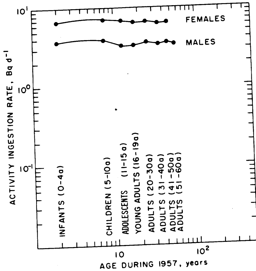
Fig. 12 Age and Sex Group Mean Values For ^{90}\text{Sr} Activity Ingestion Rate Referenced To Mid 1957 For Rongelap Atoll
